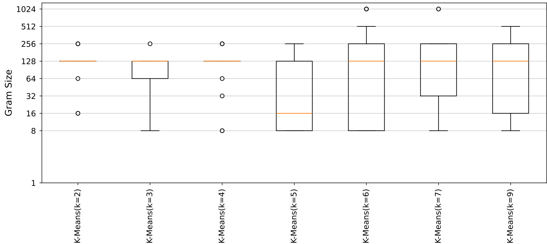
YARA Rules Gram Size Distribution (Cluster13_Size9 dataset)
